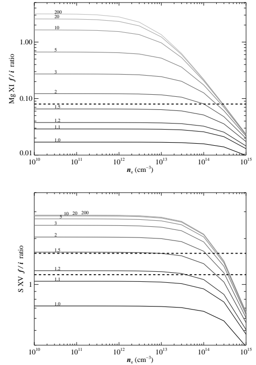
FIG. 13.— He-like f/i ratio versus n_e at various radii from 1–200 R_* , assuming a 45000 K photosphere, for Mg XI (upper panel) and S XV (lower panel). The measured f/i upper and lower bounds from Table 4 are shown as dashed lines. The Mg XI, Si XIII, and S XV suggest a formation radius, 1.2R_* \leq R \leq 1.5R_* .
