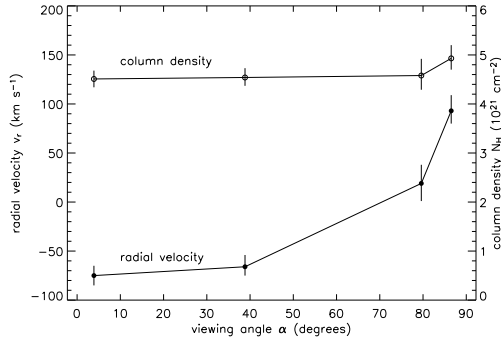
FIG. 14.— The HEG/MEG spectra show slight changes in radial velocity (left axis, filled circles) and column density (right axis, open circles) from observation to observation. At low viewing angles (pole-on), the X-ray lines are slightly blueshifted; at high viewing angles (disk-on), the lines are redshifted with a hint of excess absorption from ionized gas in the disk. The increased absorption may indicate outflowing wind material in the magnetic equatorial plane. The redshifts and blueshifts may indicate obliquely infalling material seen from various viewing angles.
