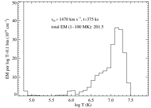
FIG. 6.— Volume emission-measure distribution per \log T = 0.1 bin, from the snapshot in Fig. 5. The MHD simulation is used to compute the emission-measure per unit volume per logarithmic temperature bin, then integrated over 3D space assuming azimuthal symmetry about the magnetic dipole axis. The total simulated volume emission measure in the interval 6.0 \leq \log T < 8.0 exceeds the total emission measure seen with the HETG by a factor of two. The low-velocity wind ( v_\infty \approx 1470 \text{ km s}^{-1} ) simulation in Fig. 5 also produces a slightly cooler distribution of shocks than observed. Full 3D MHD simulations may be needed to resolve these discrepancies.
