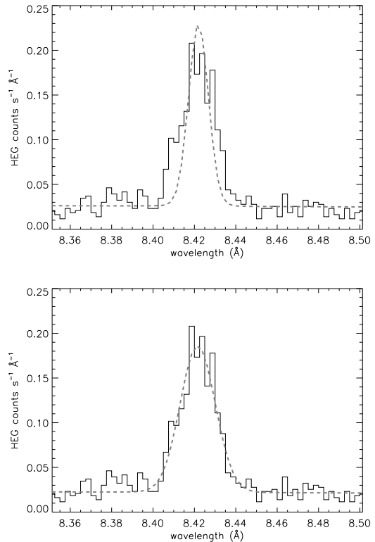
FIG. 7.— The Mg Lyman- \alpha line in the combined Chandra HEG spectrum from all four observations (solid histogram, both panels). A model with only thermal broadening ( v_{\text{th}} = 104 \text{ km s}^{-1} ; dashed line, upper panel) is much narrower than the observed profile. A Gaussian line model with thermal and turbulent broadening due to bulk motion ( \xi = 328 \text{ km s}^{-1} ; dashed line, lower panel) provides a better fit to the data.
