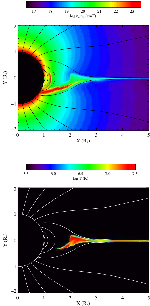
FIG. 5.— Grayscale (print edition) and color (electronic edition) snapshots from the 500-ks, slow-wind, 2D MHD simulation of \theta^1 Ori C, superposed with corresponding magnetic field lines. Upper panel: logarithm of the emission measure per unit volume, \log n_e n_H . Lower panel: logarithm of temperature, \log T . In this snapshot, obtained at simulation time t = 375 ks, material trapped in closed loops is falling back toward the stellar surface along field lines, forming a complex “snake-like” pattern. The regions of highest emission measure in the 1–100 MK temperature range occur above and below the magnetic equator, close to R \approx 2R_* .
