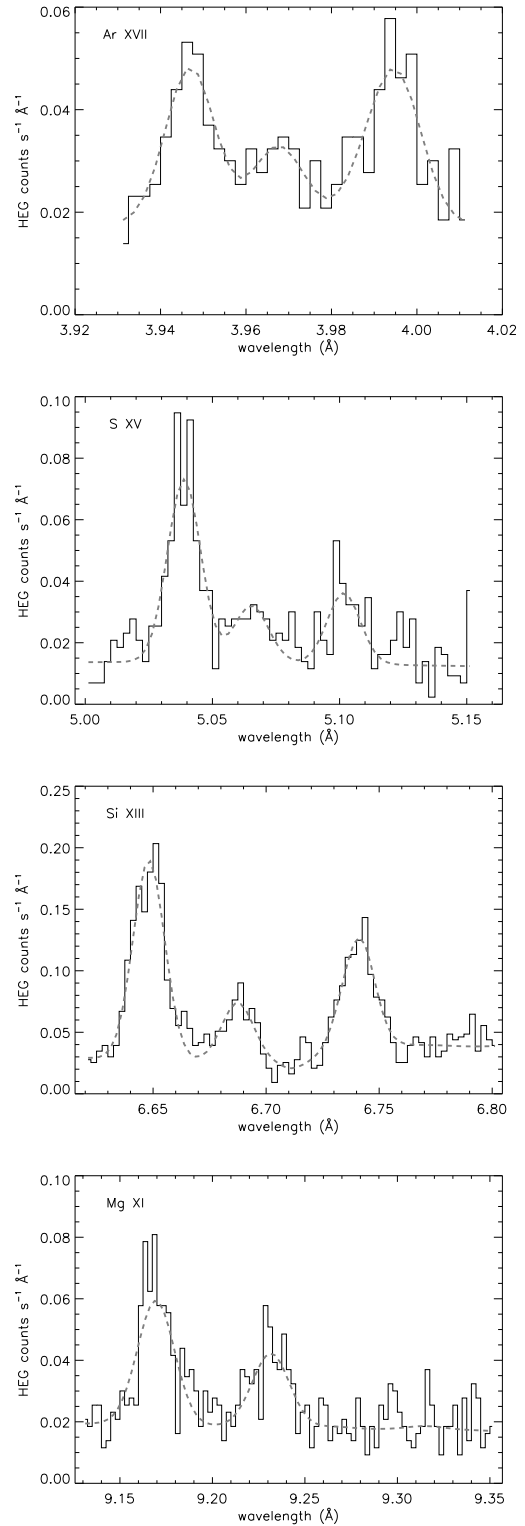
FIG. 12.— Ar XVII, S XV, Si XIII, and Mg XI He-like line complexes. In each panel, the data (solid histogram) and model (gray dashed line) of the resonance (r), intercombination (i) and forbidden (f) lines are shown. Note that as atomic number increases from Z = 12 (Mg XI) to Z = 18 (Ar XVII), the relative strength of the forbidden line to the intercombination line increases. The Si XIII f line is blended with a Mg XII line. The other detected He-like lines were not used for the diagnostic analysis: Ca XIX was too weak and the Fe XXV f and i lines were not resolved.
